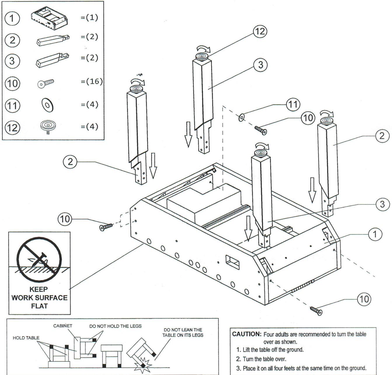
FIG. 1: LEG ASSEMBLY
